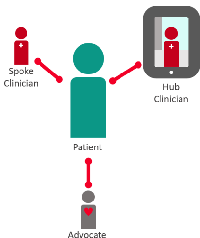
Figure 3. eSANE Program
